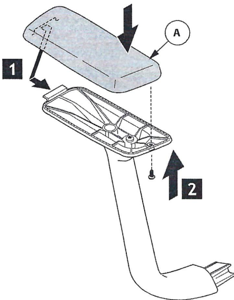
Fixed Arm
